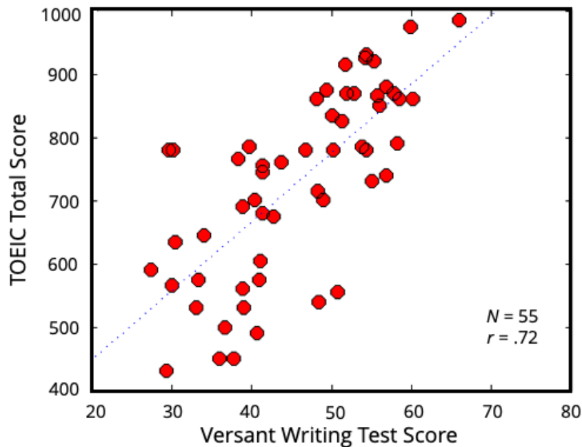
Figure 3. Scatterplot showing the relationship between the English Writing Test and TOEIC ( N = 55 ).
