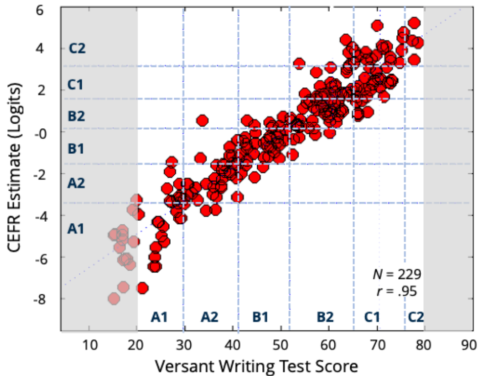
Figure 4. Scatterplot of CEFR ability estimates and English Writing Test scores
