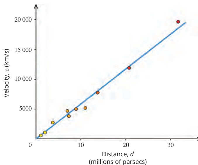
FIGURE 7.8.3 This graph shows data for the velocity of galaxies plotted against the distance to the galaxies. The resulting straight-line graph means the two values are proportional, related by a constant called the Hubble constant, H_0 .
