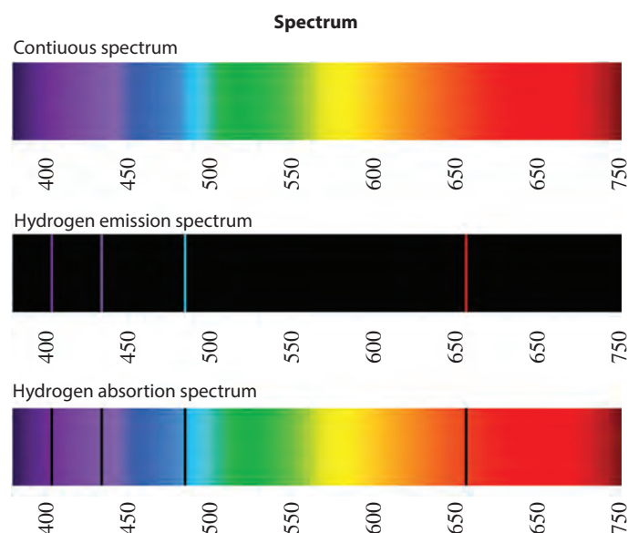
FIGURE 7.5.4 The emission and absorption spectra of hydrogen. In the emission spectrum, only light of certain wavelengths are visible. In the absorption spectrum the same wavelengths are missing and appear as black lines.
