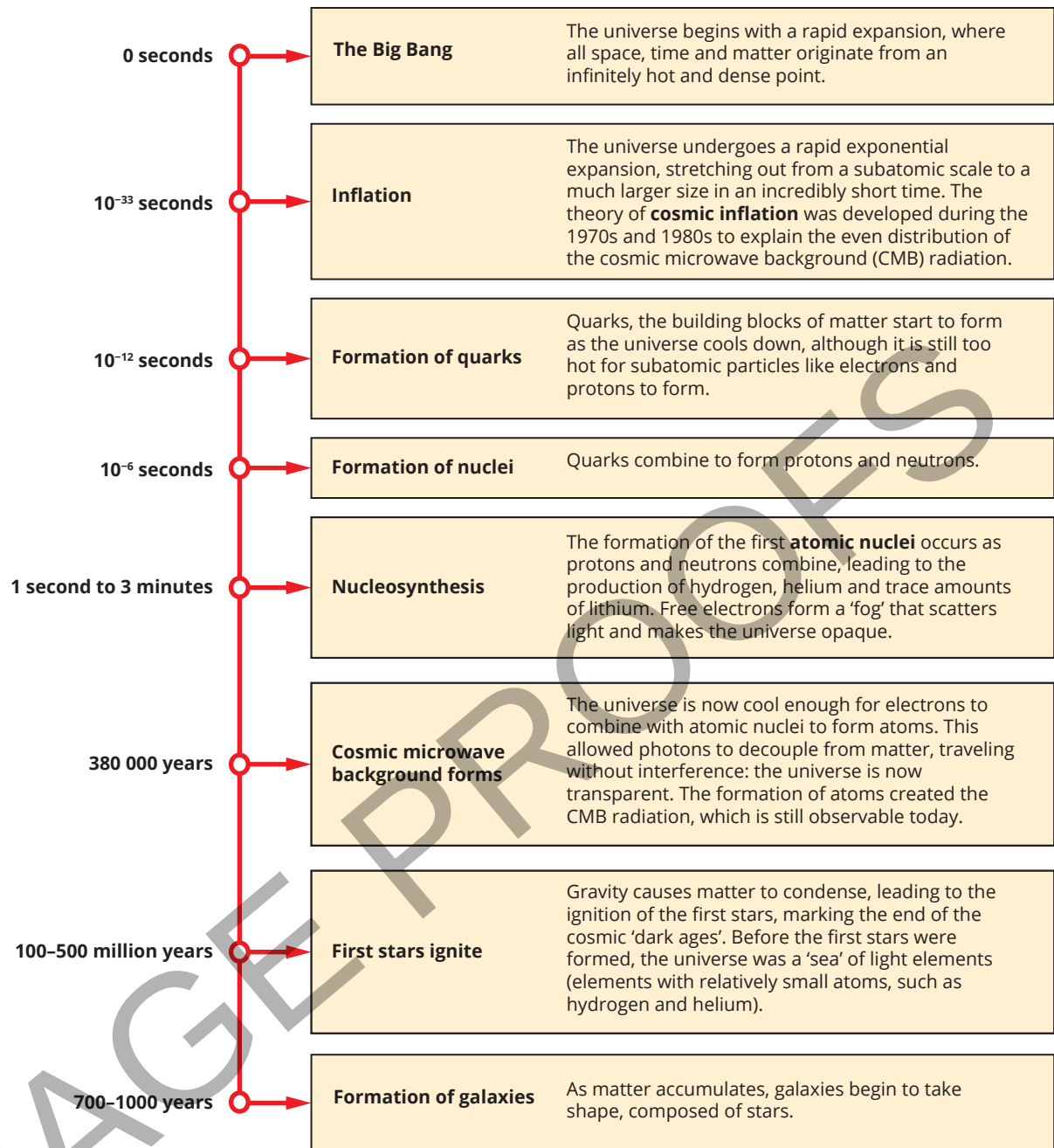
FIGURE 7.4.3 A timeline showing the development of the early universe after the Big Bang
