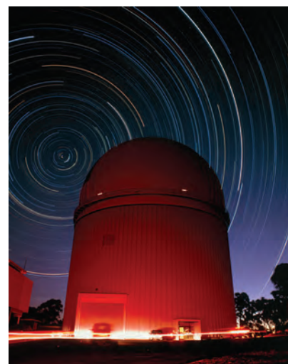
FIGURE 7.11.6 Time-lapse image of the Anglo-Australian Telescope
