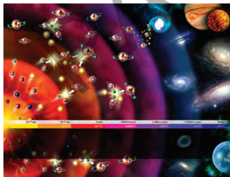
FIGURE 7.4.1 Computer artwork showing the universe's evolution from the Big Bang to the present day
