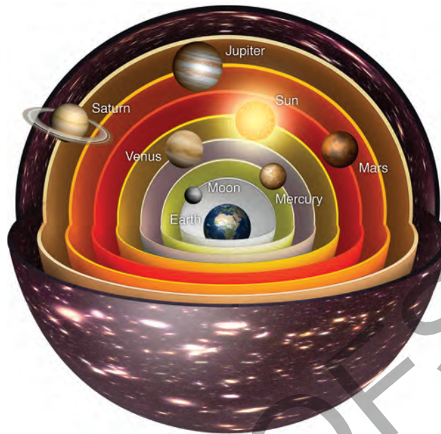
FIGURE 7.1.2 A representation of the geocentric model of the Universe, proposed by Aristotle
