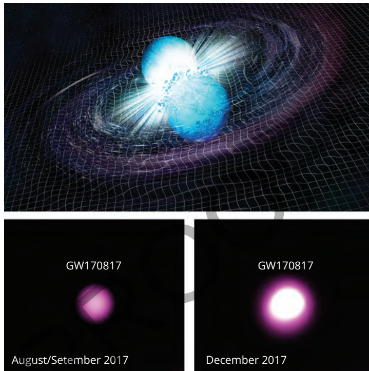
FIGURE 7.11.5 Neutron star merger. Two separate stars underwent supernova explosions, leaving behind two ultra-dense cores (neutron stars) that eventually collided (top). Gravitational wave radiation (observed by the LIGO and Virgo detectors) is shown rippling outwards from the merger. The result was a black hole.
