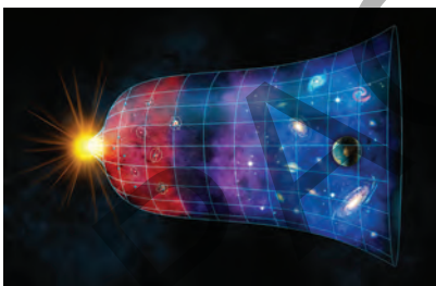
FIGURE 7.3.1 The universe has been expanding since its beginning
