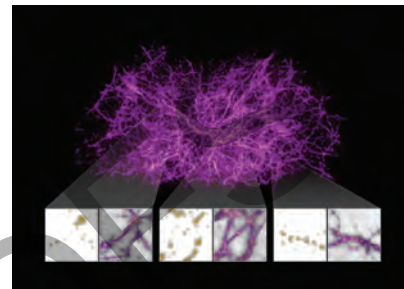
FIGURE 7.4.4 Illustration depicting the cosmic web structure of the universe, generated by a computer algorithm using data from the Sloan Digital Sky Survey
