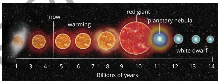
FIGURE 7.9.4 The life cycle of the Sun, a low-mass main sequence star
