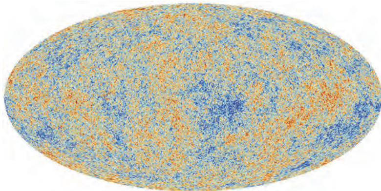
FIGURE 7.3.2 A photo from the European Space Agency of a spectacular map of the 'oldest light' in the sky: the cosmic microwave background radiation (CMB) as observed by the Planck telescope. This photo shows tiny temperature fluctuations that correspond to regions of slightly different densities, representing the seeds of all future structure: the stars and galaxies of today.
