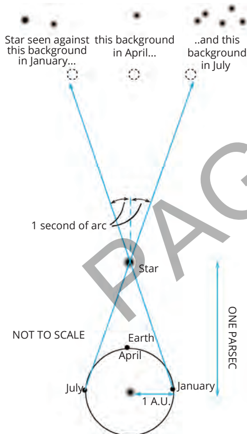
FIGURE 7.2.3 A nearby star viewed from either side of Earth's orbit (lower centre), the largest possible baseline
