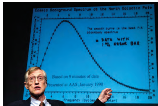
FIGURE 7.3.4 Dr John Cromwell Mather (born 1945), American astrophysicist, cosmologist and Nobel laureate, talking at a press conference about the work he did that helped show the blackbody nature of cosmic microwave background radiation. He was awarded a share of the 2006 Nobel Prize in physics for this work.
