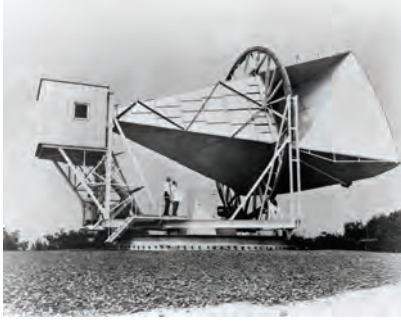
FIGURE 7.3.3 The horn antenna at Bell Telephone Laboratories in Holmdel, New Jersey, USA, which astrophysicists Wilson and Penzias used in 1963–64 to unexpectedly discover the microwave background radiation from the Big Bang.
