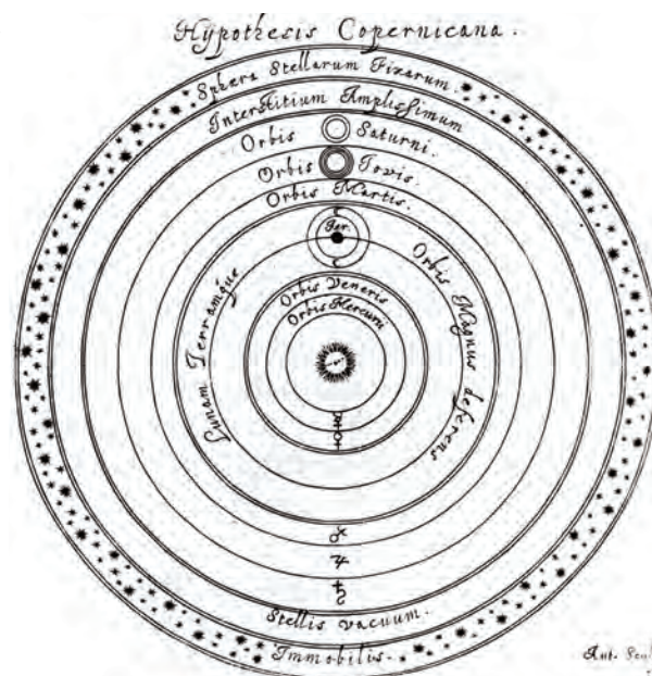
FIGURE 7.1.3 Copernican (heliocentric) system of the universe, showing the orbits of the planets surrounded by the firmament of the fixed stars. From Selenographia by Johannes Hevelius. (Gdansk, 1647). Artist: Johannes Hevelius.
