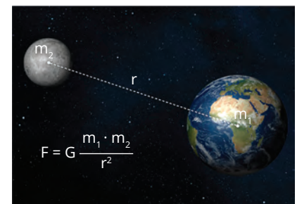
FIGURE 7.1.5 The equation for Newton's law of gravitation applied to the Earth-Moon system
