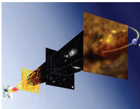
FIGURE 7.4.2 The four stages of the expansion of the universe.
