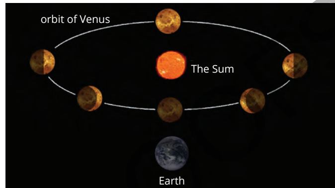
FIGURE 7.1.6 This diagram shows how a heliocentric structure of the solar system explains the phases of Venus as seen from Earth.
