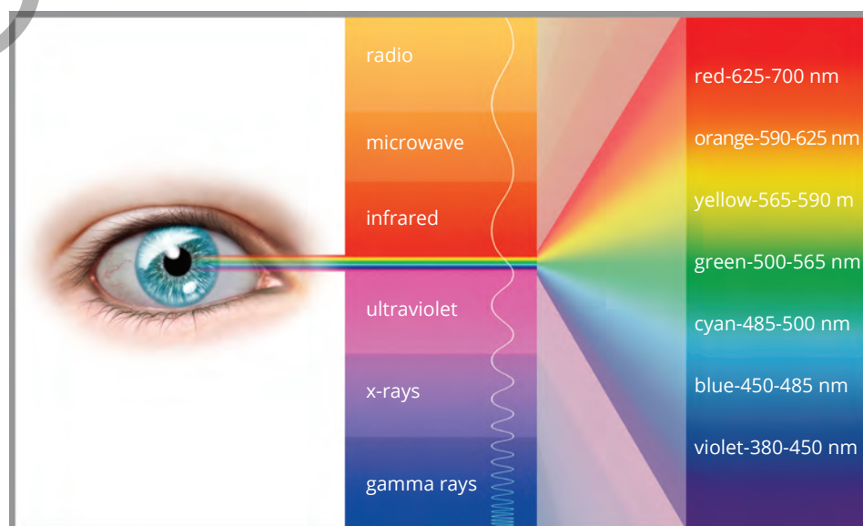
FIGURE 7.5.2 The electromagnetic spectrum. Light is separated into different groups based on specific wavelengths and frequencies.
