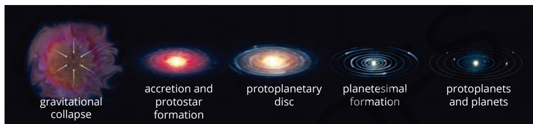
FIGURE 7.4.5 Formation of a solar system
