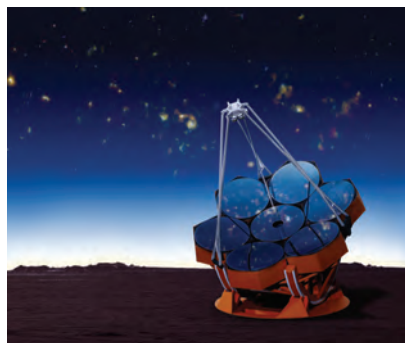
FIGURE 7.11.7 Artwork of the Giant Magellan Telescope (GMT), an optical telescope comprising seven primary mirrors, each with a diameter of 8.4 metres
