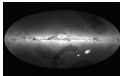
FIGURE 7.2.4 All-sky map of the Milky Way and neighbouring galaxies from observations of the Gaia satellite. Brighter regions indicate denser concentrations of stars and darker regions fewer stars. The Galactic Plane of the Milky Way is seen across the centre. This is about 100 000 light years across and about 1000 light years thick.
