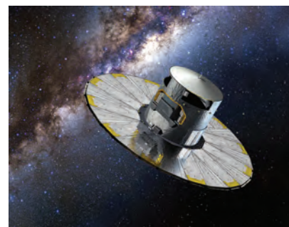
FIGURE 7.8.4 The GAIA mission, launched by the European Space Agency (ESA), aims to map the positions, distances, and velocities of over a billion stars in the Milky Way galaxy and beyond.
