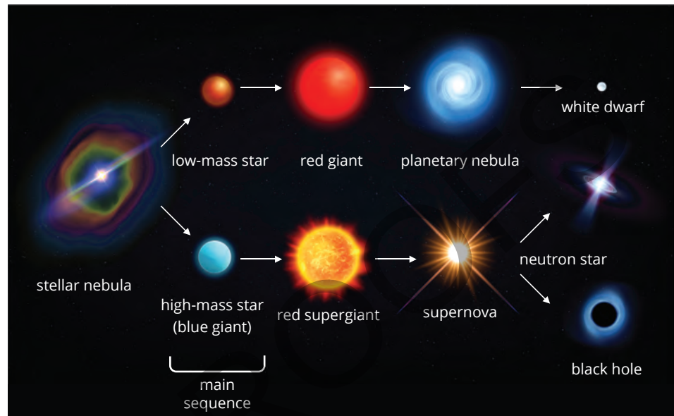
FIGURE 7.9.2 Illustration of the life cycle of a star showing different paths, depending on the initial mass of the star
