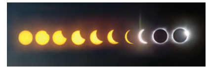
FIGURE 7.1.7 A series of images taken during a total solar eclipse
