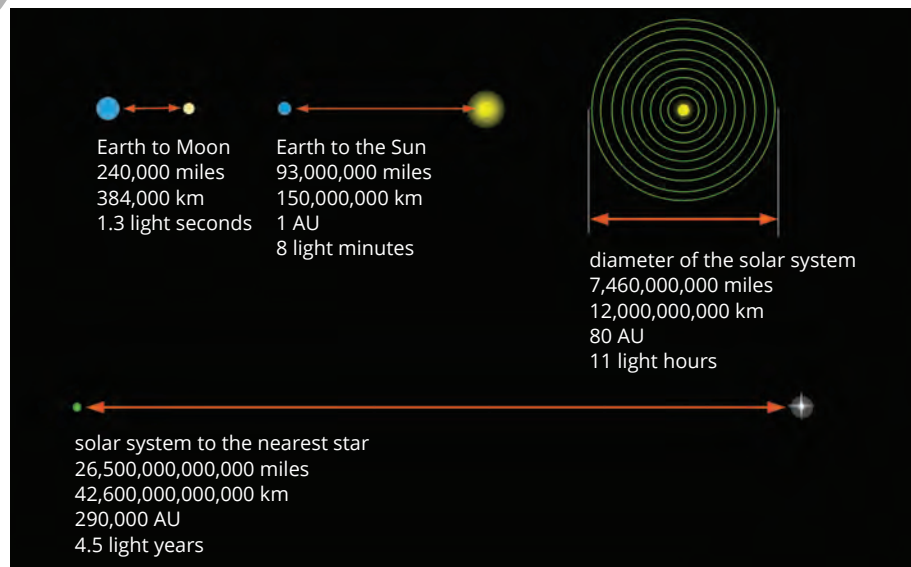
FIGURE 7.2.2 Comparing units of measurement for describing distances in space
