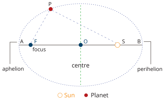
FIGURE 7.1.4 Kepler's first law of planetary motion says that all planets (shown as P) move around the Sun (shown as S) in an elliptical orbit, where the Sun is at one foci of the ellipse.
