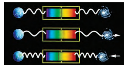
FIGURE 7.8.2 Evidence for an expanding universe includes the redshift observed in light travelling from distance galaxies.
