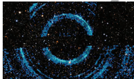
FIGURE 7.9.7 Composite X-ray (light blue) and optical image of rings around a black hole in V404 Cygni. In 2015, X-ray flares were detected from the black hole producing high energy rings known as light echoes. The light echoes were created when light reflected off dust clouds between V404 Cygni and Earth, forming the concentric rings.
