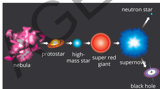
FIGURE 7.10.1 A neutron star is produced at the end of a life cycle of a large star
