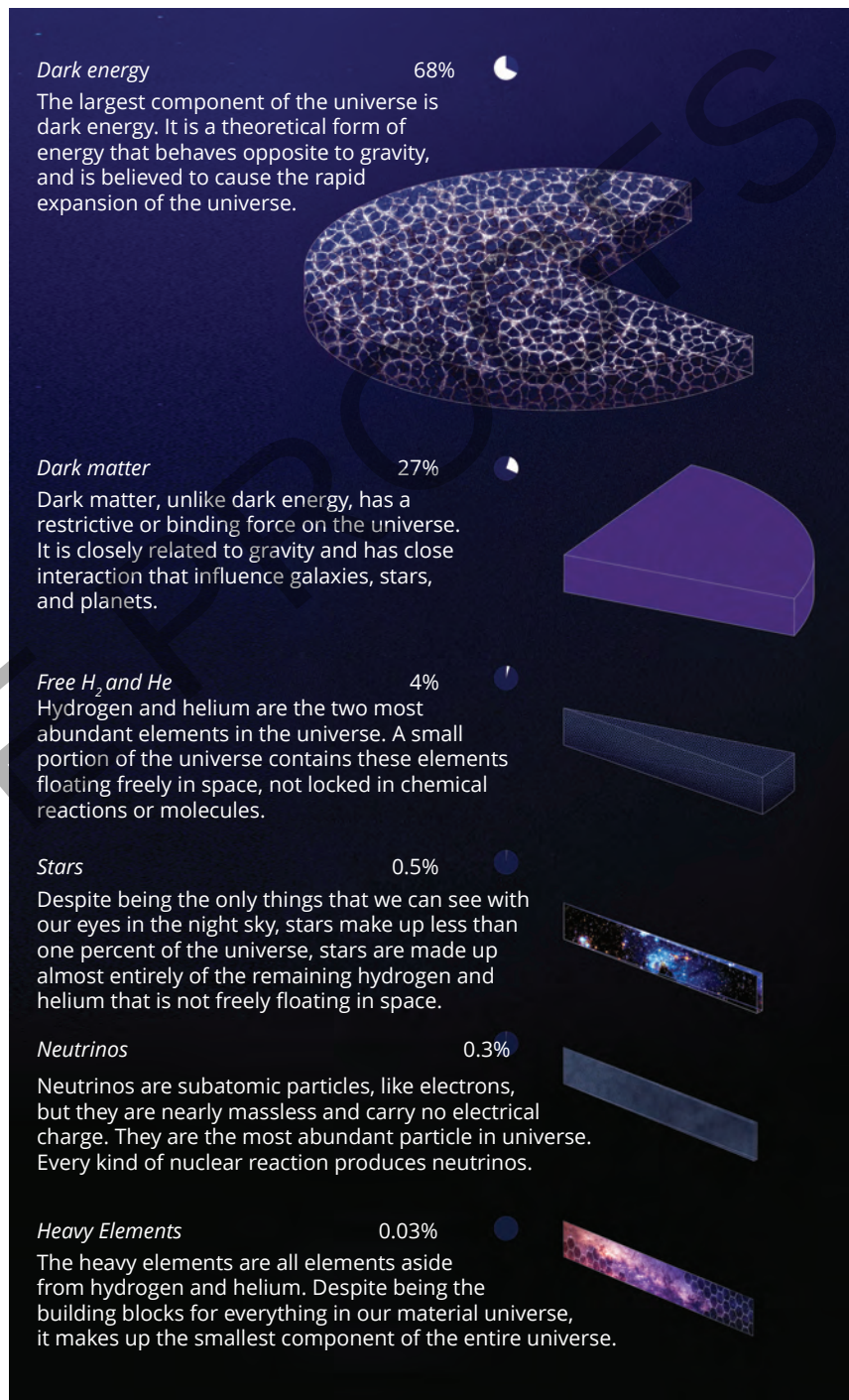
FIGURE 7.11.2 Infographic illustration depicting the contents of the universe. Data based on measurements by the European Space Agency and the Brookhaven National Observatory.
