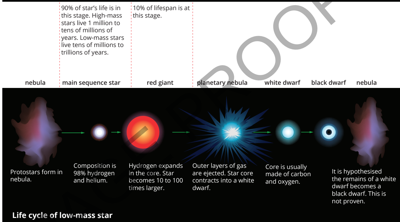
FIGURE 7.9.3 Stars follow different lifecycles depending on their initial mass
