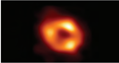
FIGURE 7.9.6 Event Horizon Telescope (EHT) collaboration image of Sagittarius A*, the supermassive black hole at the centre of the Milky Way. Image taken using 2017 observations from the Event Horizon Telescope (EHT), a global network of radio telescopes.
